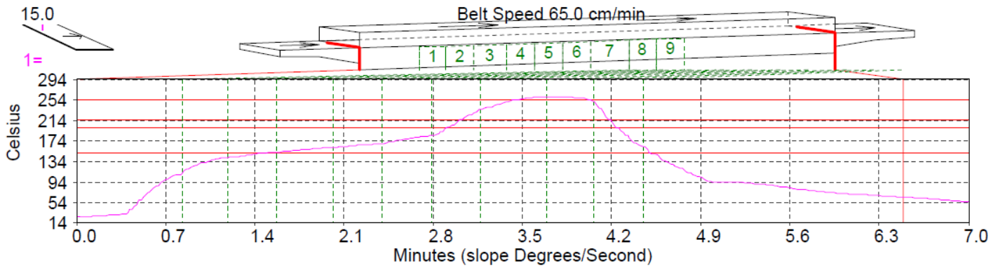
Figure 1 Lead-free Solder Temperature Reflow Profile and Belt Speed for Crocus Products
