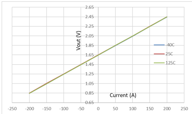
FIGURE 6 TRI-TEMP PERFORMANCE OF CTD453 WITH BUSBAR
